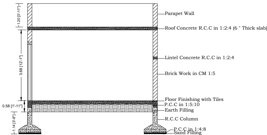
SECTION X-X
