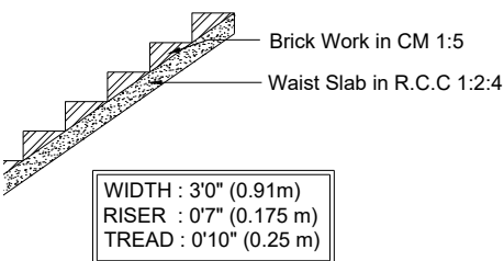
STAIRCASE DETAILS
