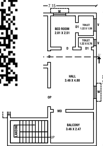
FIRST FLOOR PLAN (PROPOSED BUILDING)
