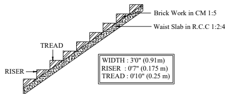
STAIRCASE DETAILS
