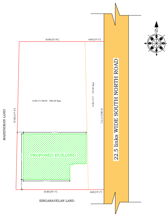
SITE PLAN (SCALE -1:250)
