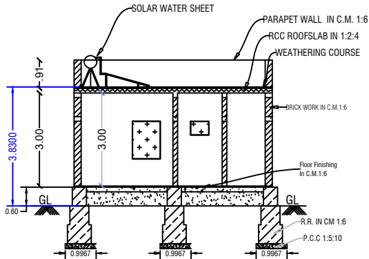
SECTION ON-"AB"
