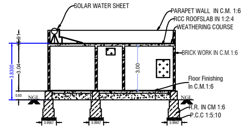
SECTION ON-"AB"
