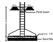
FOUNDATION DETAILS
