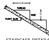
STAIRCASE DETAILS
