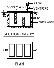
SEPTICTANK DETAILS
