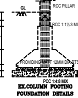
FOUNDATION DETAILS
