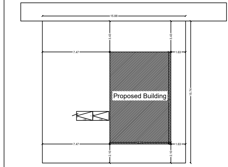
SITE PLAN SCALE 1:100 & As Per FMB
