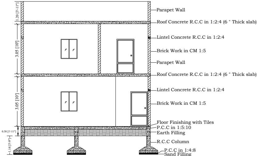
SECTION X-X
