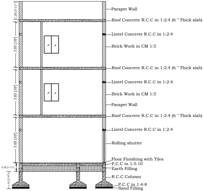
SECTION X-X
