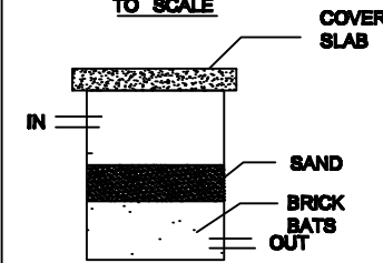
RAIN WATER DETAIL NOT TO SCALE
