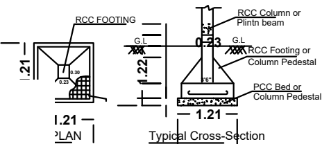
FOOTING DETAILS
