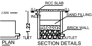
RAINWATER HARVESTING SYSTEM
