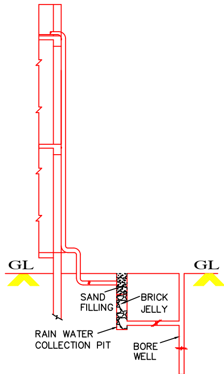
RAIN WATER HARVESTING SYSTEM
