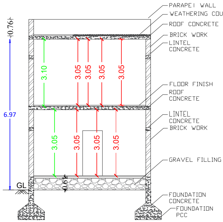
TYPICAL CROSS SECTION
