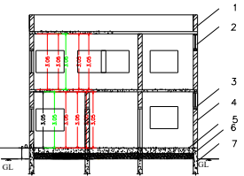
SECTION ON 'AAA'
