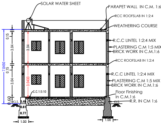
Section On-"AB"
