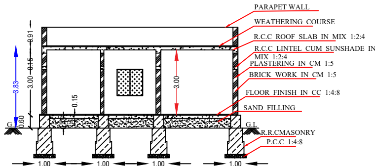
SECTION ON-"AB"
