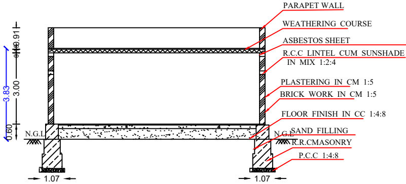
SECTION ON-"AB"
