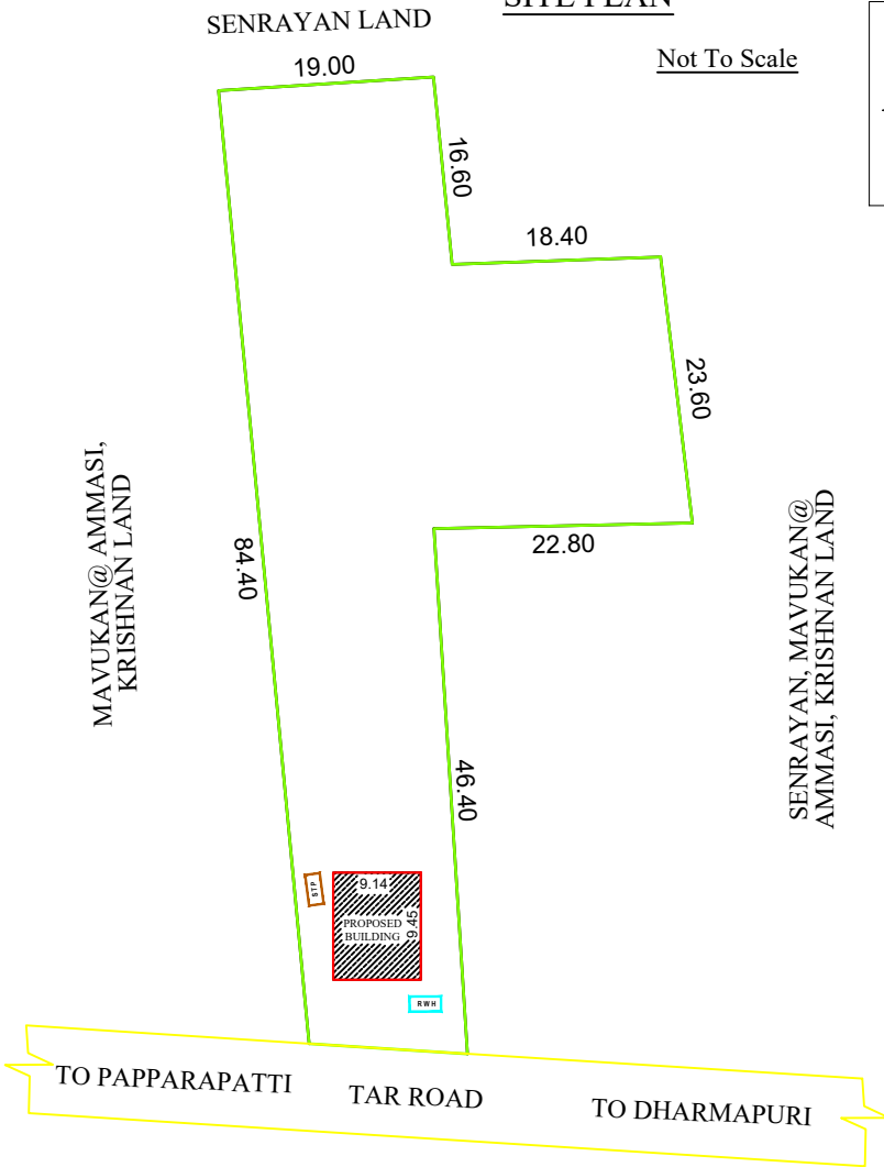
SITE PLAN
