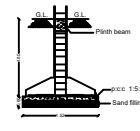
FOUNDATION DETAILS
