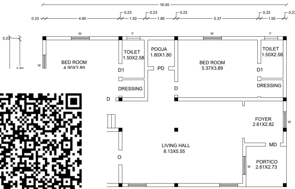
GROUND FLOOR
