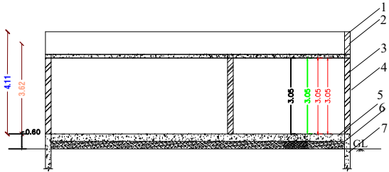
SECTION ON 'MS'
