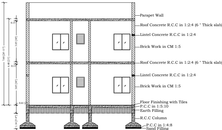
SECTION X-X
