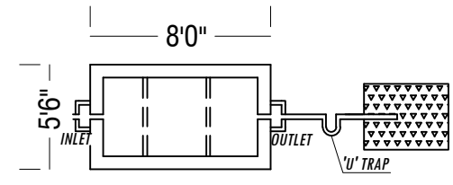
SEPTIC TANK AND DISPERSION TRENCH DETAILS
