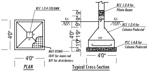
FOOTING DETAILS
