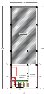
SECOND FLOOR PLAN
