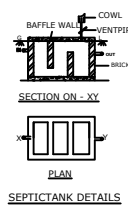
SEPTIC TANK DETAILS NOT TO SCALE
