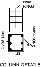
COLUMN DETAILS
