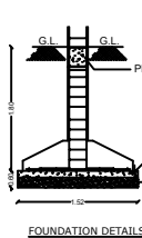
FOUNDATION DETAILS
