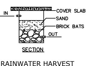
RAINWATER HARVEST NOT TO SCALE
