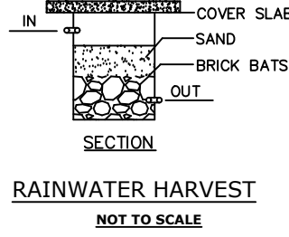
RAINWATER HARVEST NOT TO SCALE
