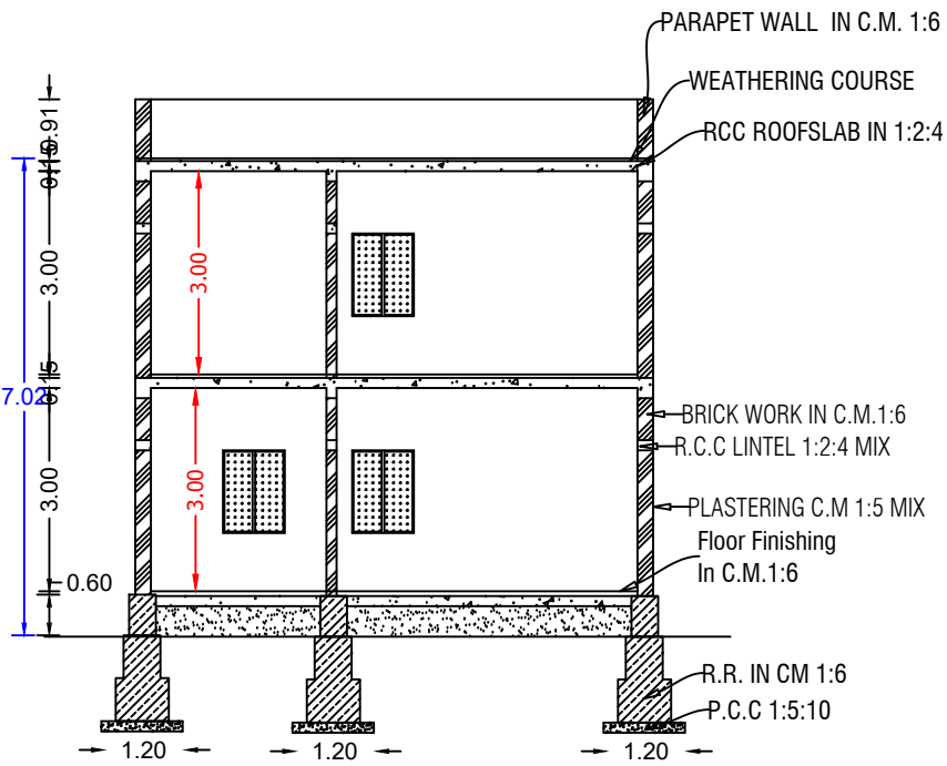
SECTION ON-"AB"
