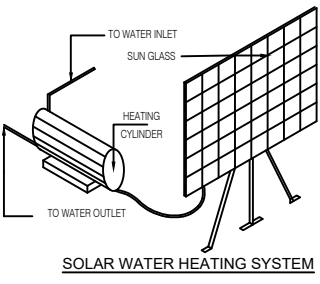
SOLAR WATER HEATING SYSTEM SCALE: 1:15
