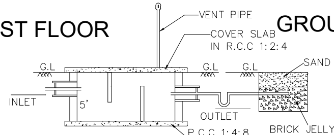
SECTION-AB
