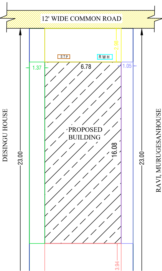
SITE PLAN
