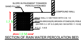
SECTION OF RAIN WATER PERCOLATION BED
