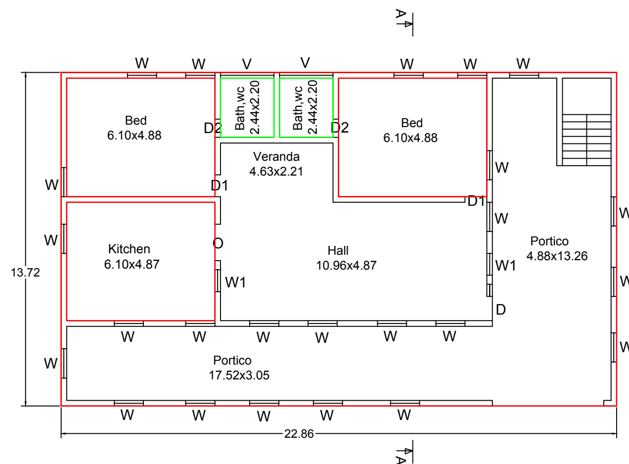
PLAN
