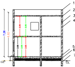
SECTION ON 'AAA'
