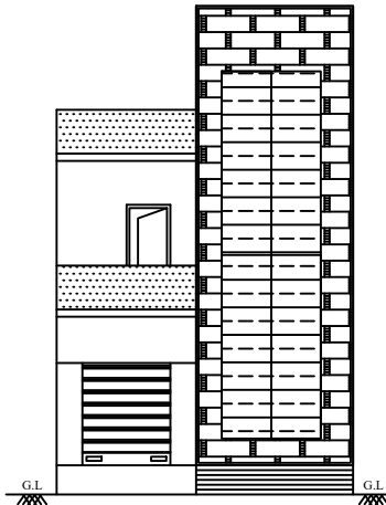
Elevation Plan
