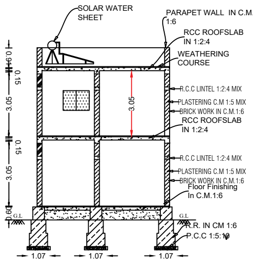
Section On-"AB"
