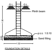
FOUNDATION DETAILS
