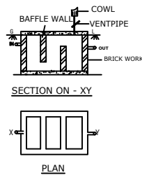
SEPTICTANK DETAILS
