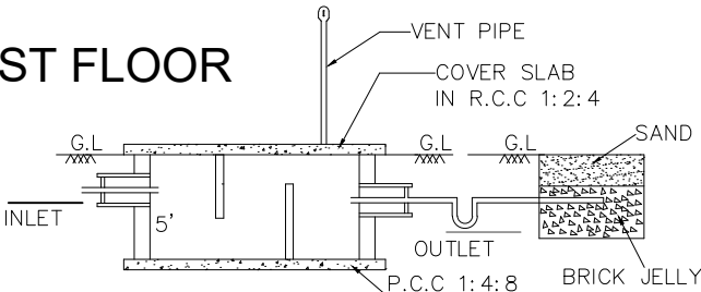
SECTION-AB
