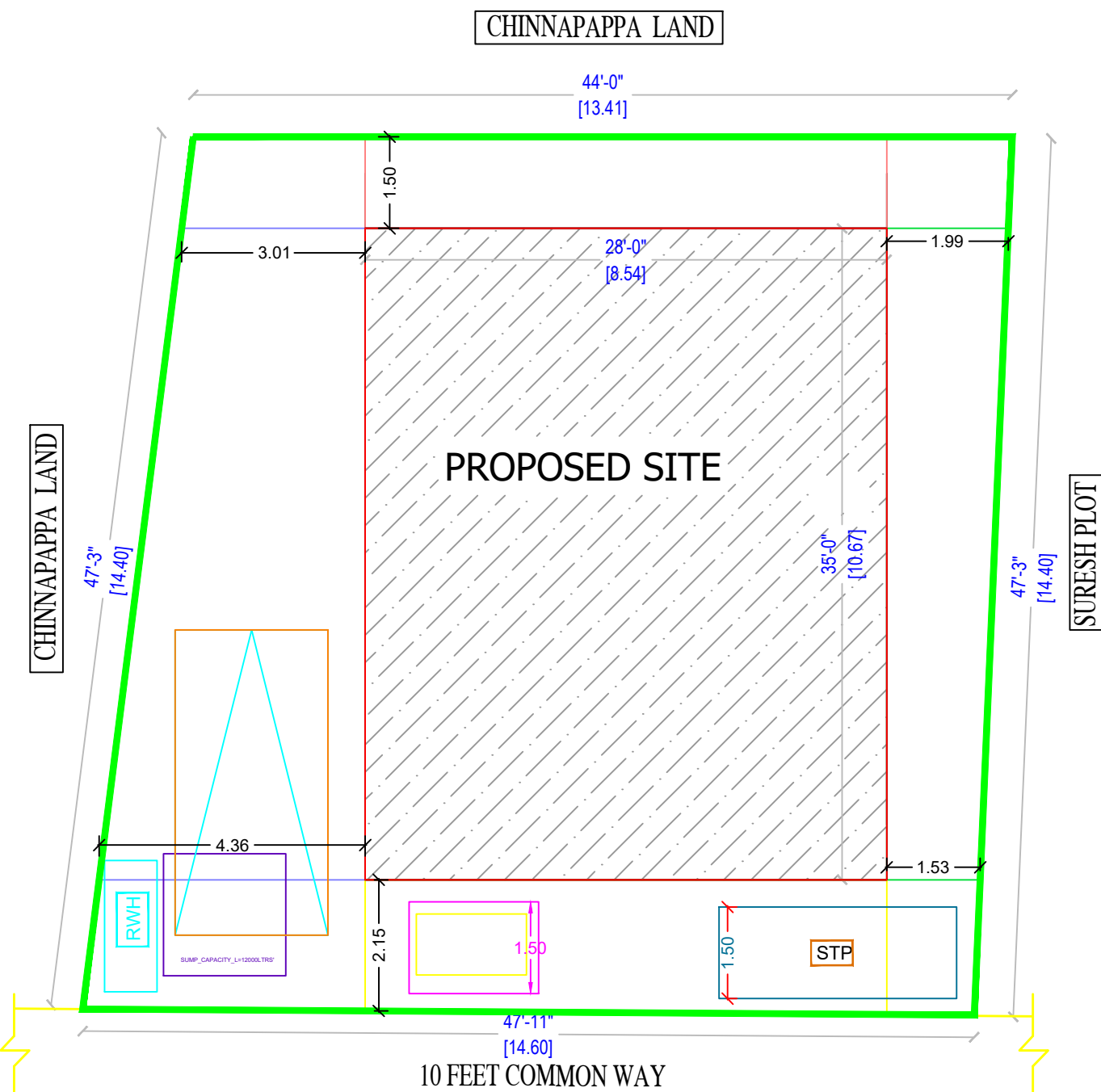
SITE PLAN
