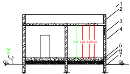
SECTION ON 'AA'
