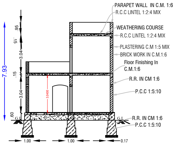
SECTION ON-"AB"
