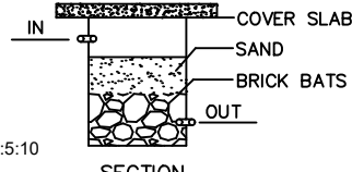
RAINWATER HARVEST NOT TO SCALE
