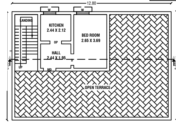
FIRST FLOOR PLAN (PROPOSED BUILDING)
