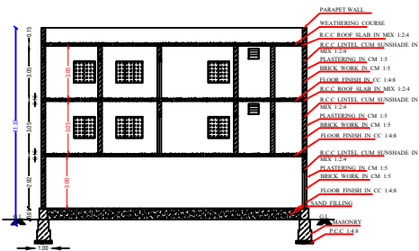
SECTION ON-'AB'
