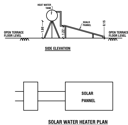
SOLAR WATER HEATER PLAN
