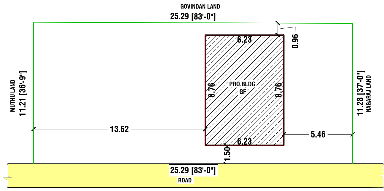
SITE PLAN
