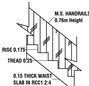
STAIRCASE DETAILS
