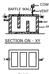
SEPTICTANK DETAILS
