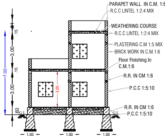
SECTION ON-'AB'
