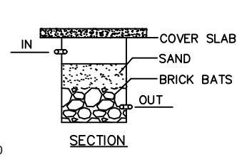
RAINWATER HARVEST
