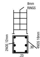
COLUMN DETAILS
