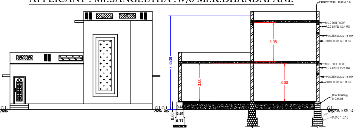
ELEVATION PLAN
