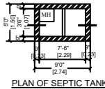
PLAN OF SEPTIC TANK
