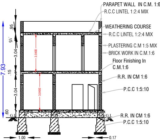
SECTION ON-'AB'
