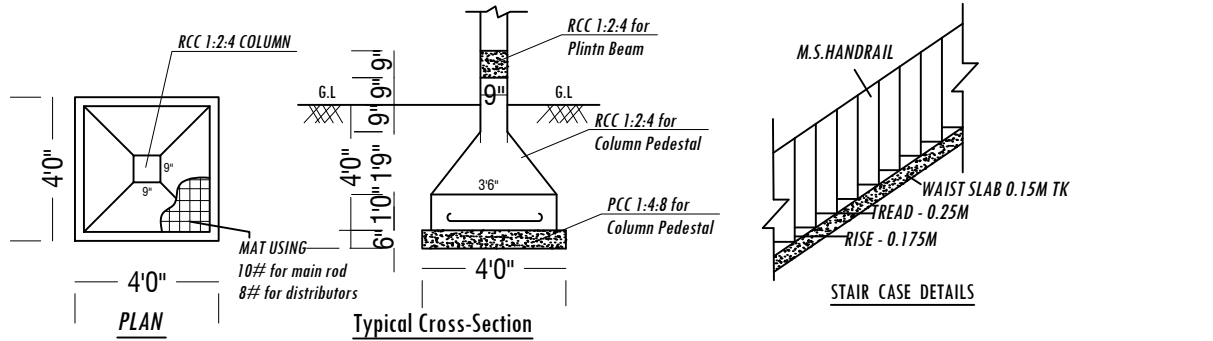
FOOTING DETAILS
