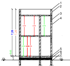
SECTION ON 'AA'
