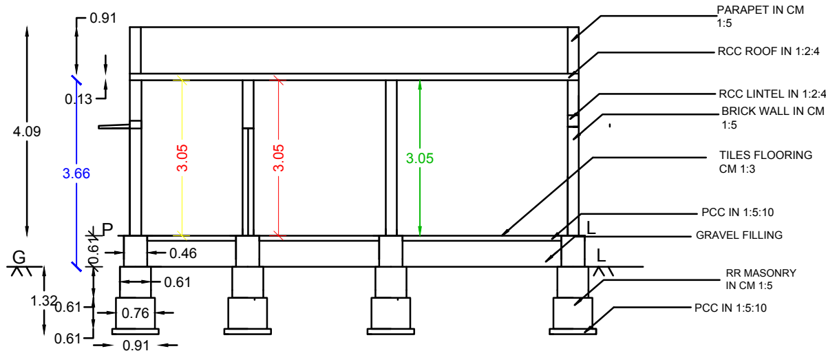
SECTION : "B-B"
