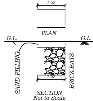
DETAILED PLAN OF RAINWATER PERCOLATION PEBBLE BED RW_H_CAPACITY_L = 2000LTRS
