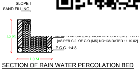
SECTION OF RAIN WATER PERCOLATION BED
