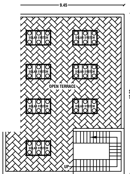
OPEN TERRACE PLAN
